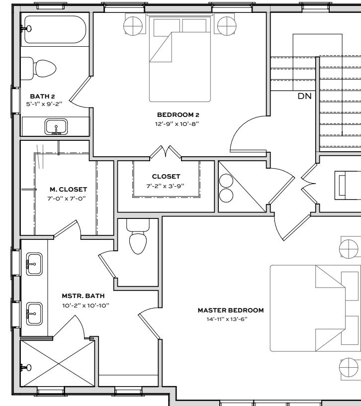
SECOND FLOOR 66 SQ. FT.
