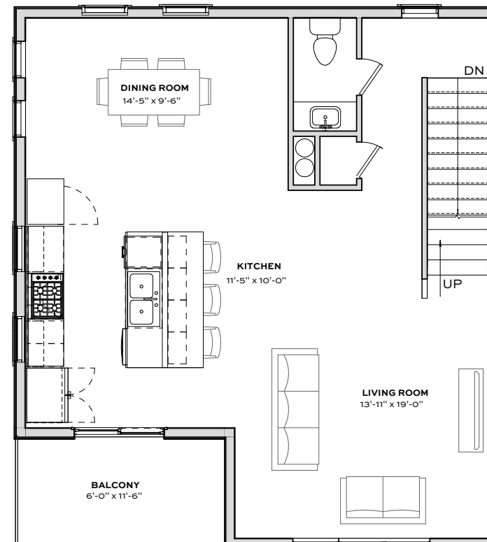
MAIN FLOOR 667 SQ. FT.
