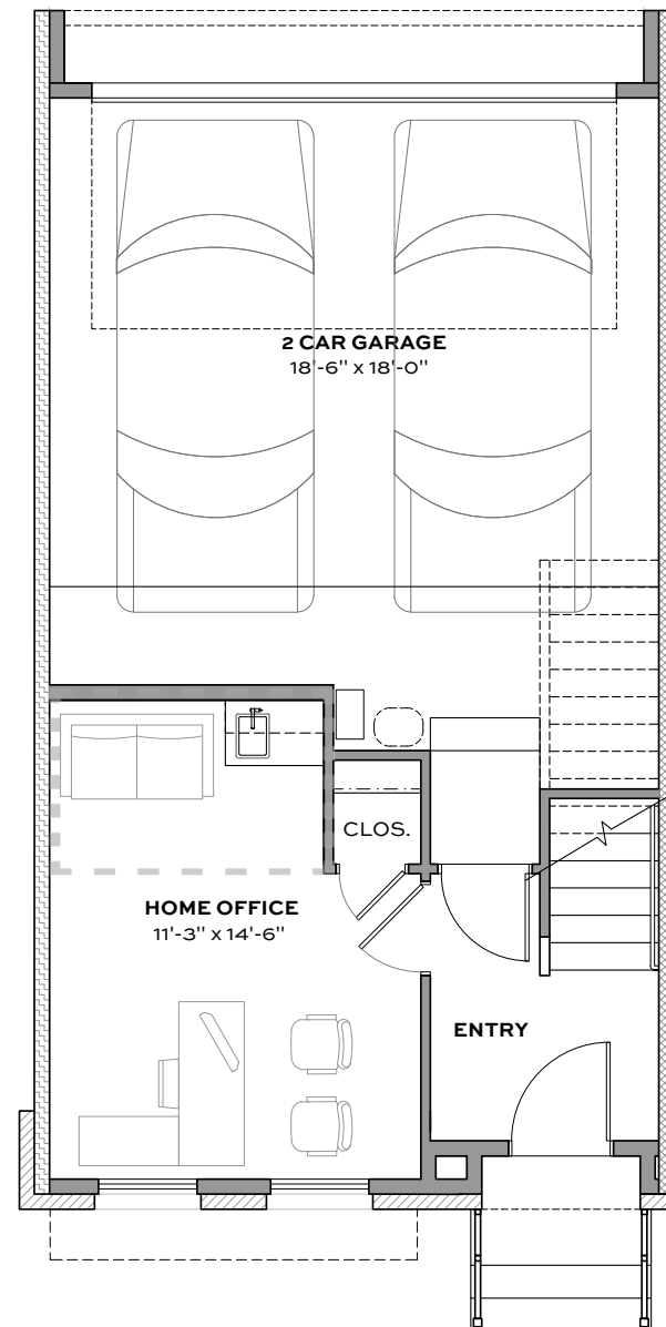
FIRST FLOOR 273 SQ. FT.
